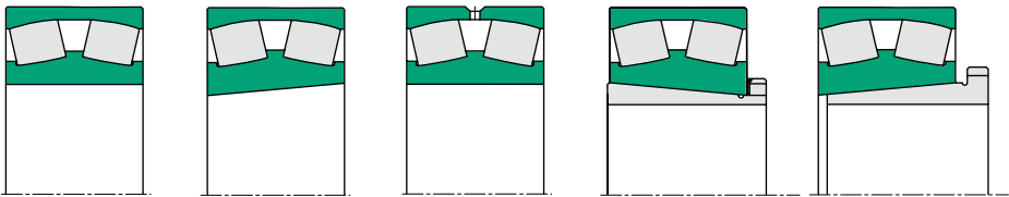
Cylindrical bore
